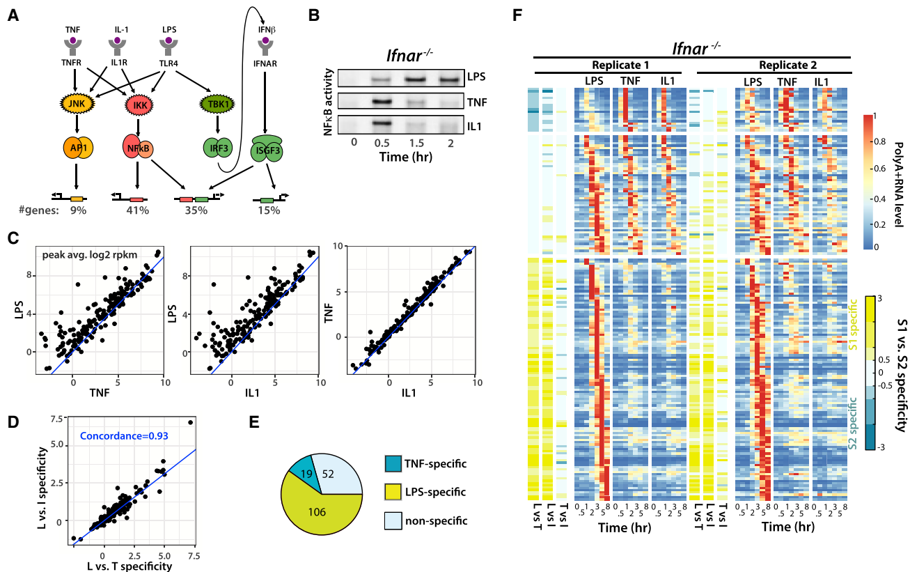
Figure 1. Identifying LPS-Specific Genes that Do Not Depend on Interferon Signaling
