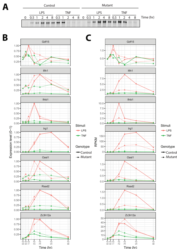
Figure S2. Related to Figure 2. (A) NF \kappa B activity measured by EMSA after pulse stimulation with LPS and TNF in control and mutant showed extended activity in mutant with TNF. (B) Line graphs of 7 genes re-categorized from group II to group I. Expression values are scaled to the maximum of each genotype under LPS or TNF stimulation. The elevated basal expression levels in the mutant initially caused these genes to be incorrectly categorized into group II. However, visual inspection shows that these 7 genes have stimulus specificity that is not dynamics dependent, and should therefore be categorized into group I. (B) Unscaled RPKM expression values.
