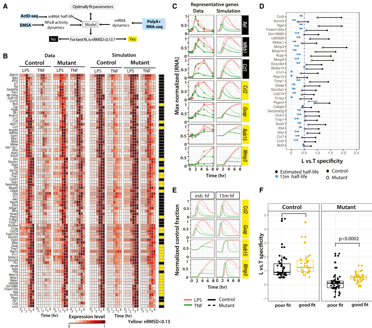
Figure 4. Model-Aided Analysis to Determine Sufficiency of mRNA Half-Life as the Decoding Mechanism
