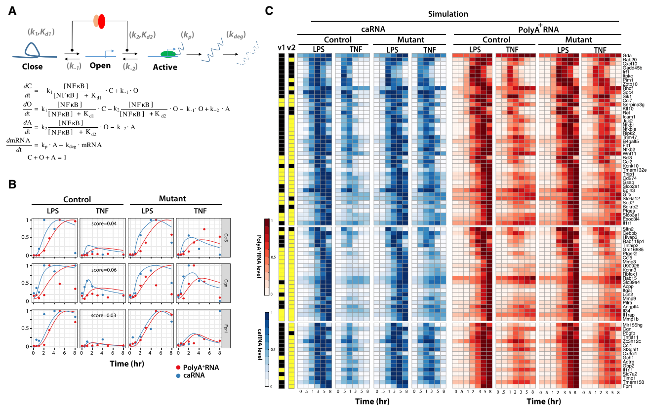
Figure 6. Model-Aided Analysis to Quantify Chromatin-Associated Decoding of Stimulus-Specific NFκB Dynamics
