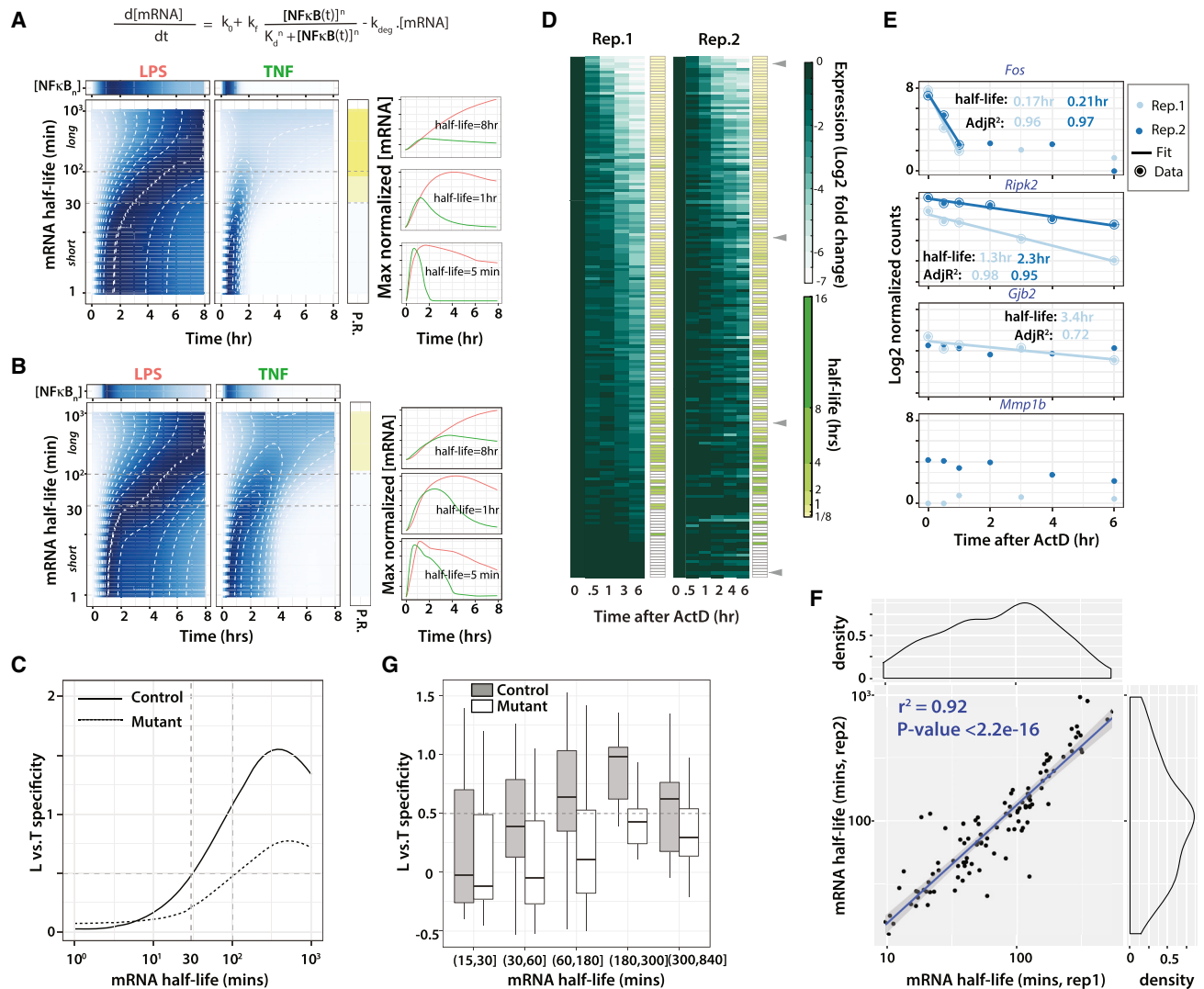
Figure 3. Long mRNA Half-Lives Are Correlated with LPS Specificity
