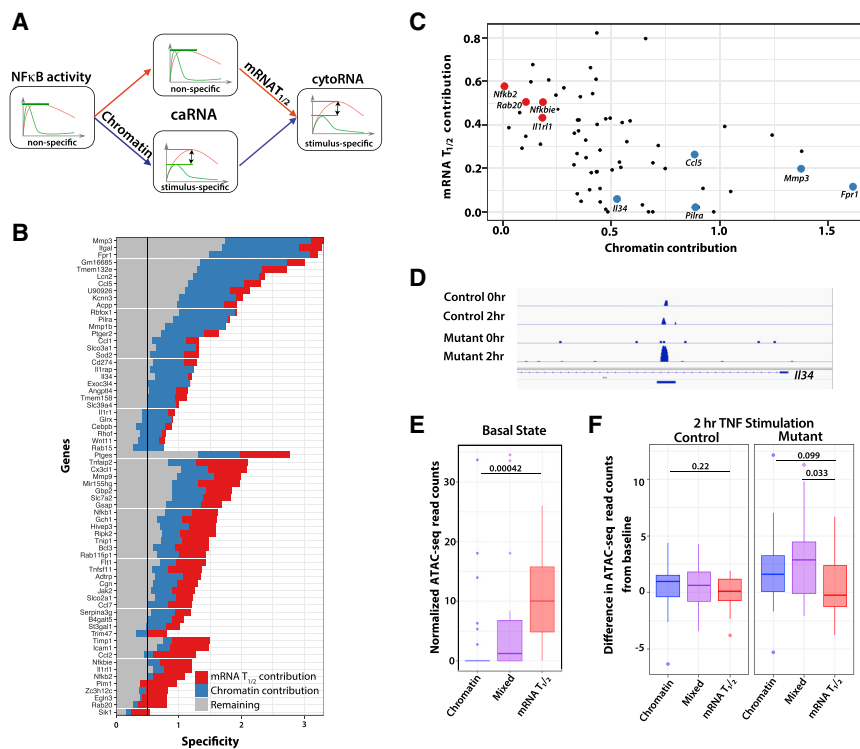
Figure 7. Distinct Regulatory Strategies that Decode NF \kappa B Duration-Dependent Gene Expression
