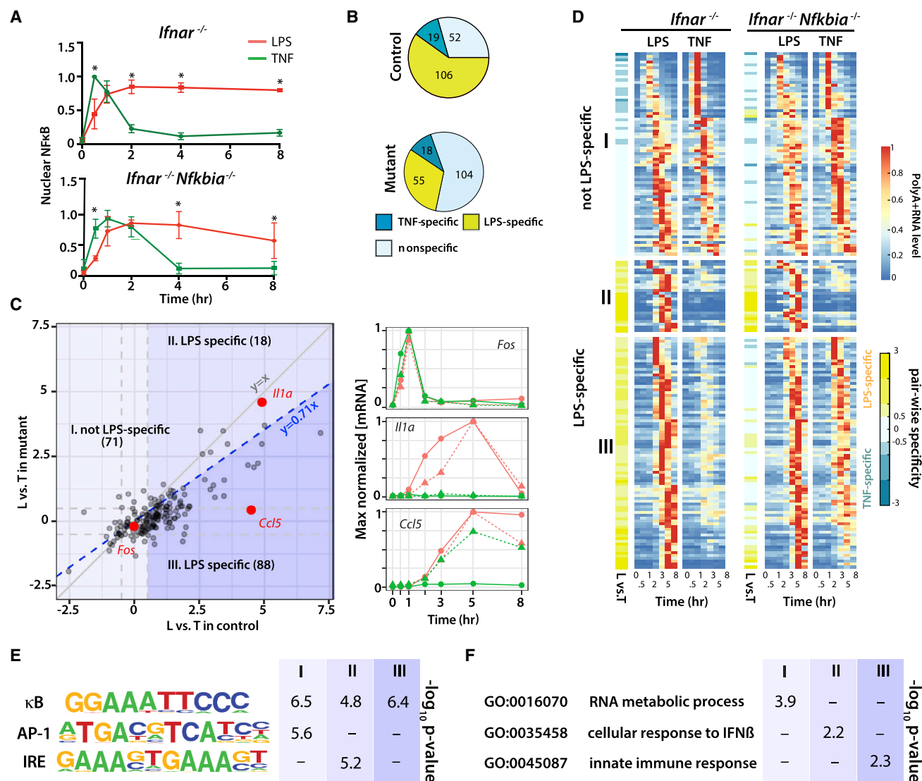
Figure 2. Determining the NFκB Duration Dependency of LPS-Specific Gene Expression
